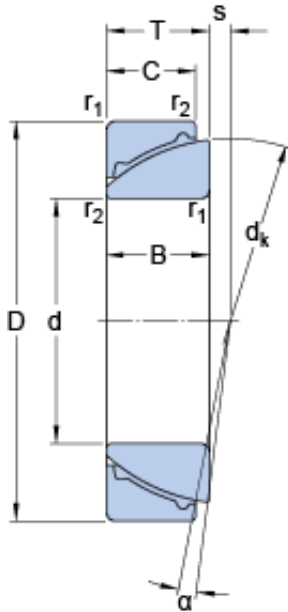
GAC 100 F Bearing 2D drawings and 3D CAD models
